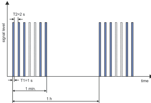
Fig. 48. An example of low-frequency signal transmission.
