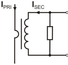
Fig. 44. CT probes with voltage output
