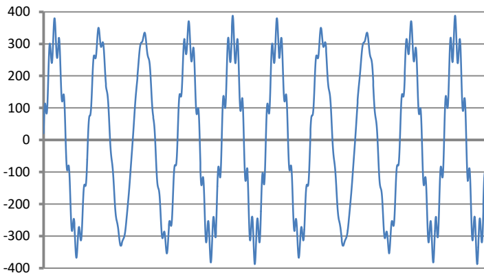
Fig. 47. The effect of 9th harmonic interaction (450 Hz, 10% Unom) and interharmonic 460 Hz (10% Unom). The apparent change in the voltage envelope with frequency of 10Hz that may cause flicker (Unom = 230 V RMS, 50 Hz).
